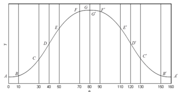
Figure 9: Sectional modified trapezoidal lift curve
