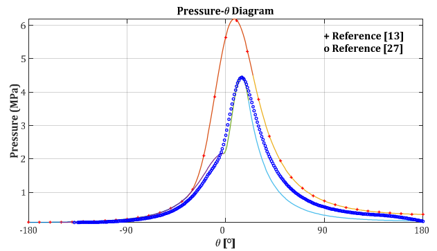
Figure 12: Pressure vs. crank angle results
