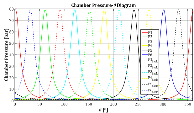
Figure 16: Chamber pressures for a 6 vane AVRE
